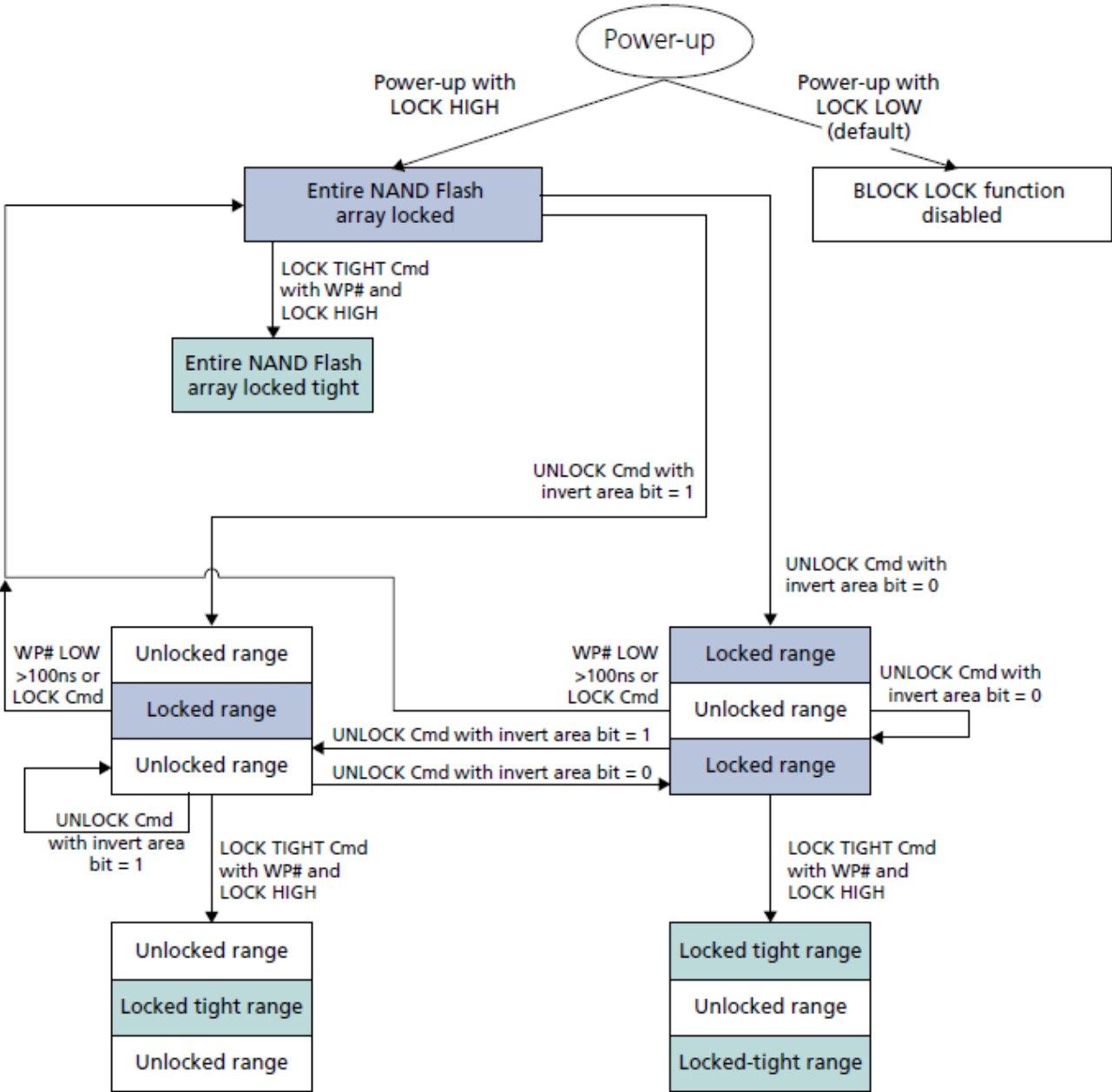
BLOCK LOCK Flowchart
