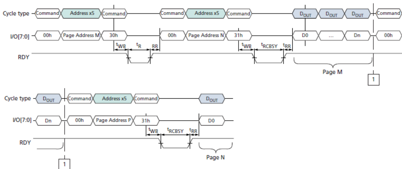
READ PAGE CACHE RANDOM (00h-31h) Operation
